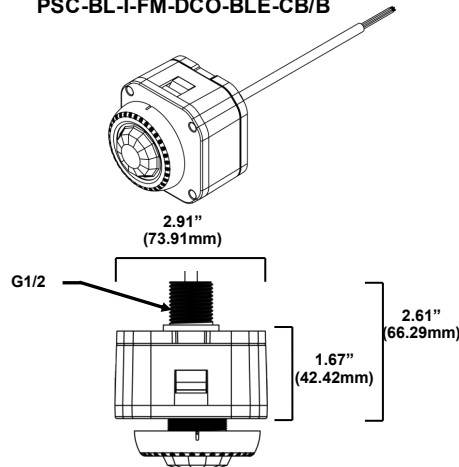
Bottom Mount Housing PSC-BL-I-FM-DC0-BLE-CB/B
