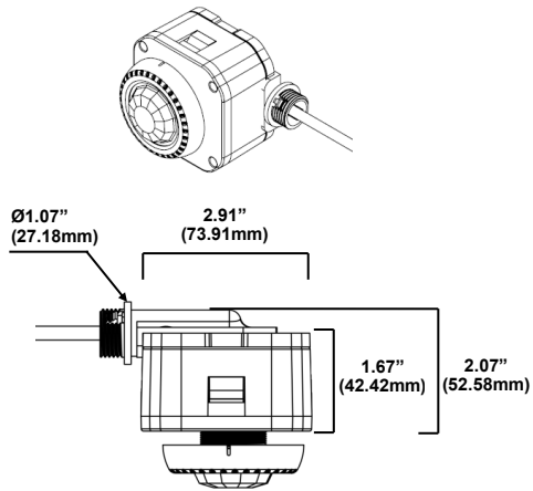
Side Mount Housing PSC-BL-I-FM-DC0-BLE-CB/S
